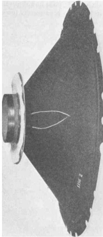
FIG. 5. Replacement cone and voice coil assembly for 515 low-frequency loudspeaker.
